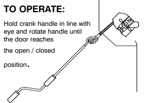
Internally installed shutter with internal manual override
