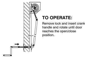
Internally installed shutter with external manual override
